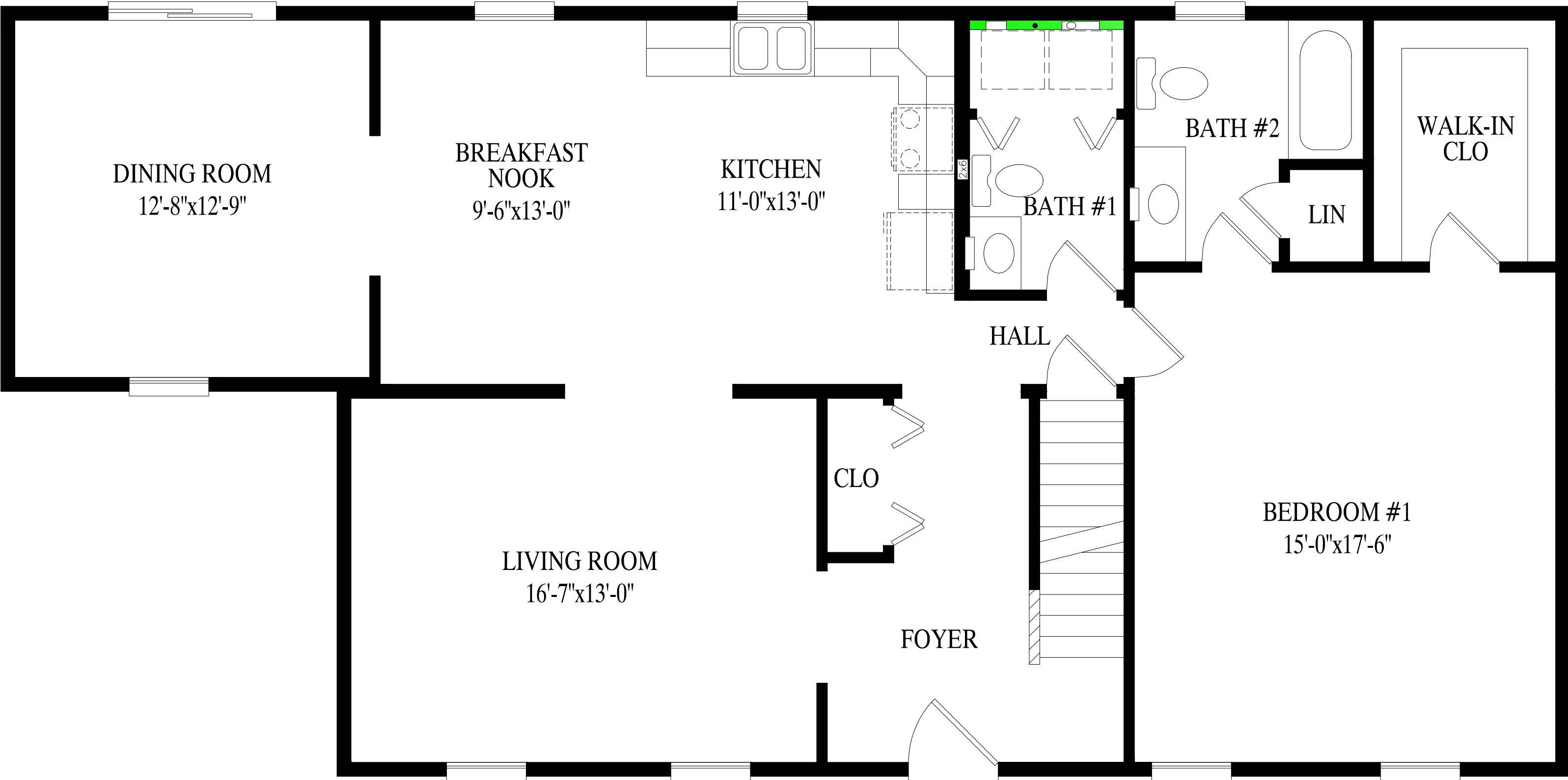
Cameron III 27' 6" X 44' 56" Cape 1375 sq. ft. first floor
